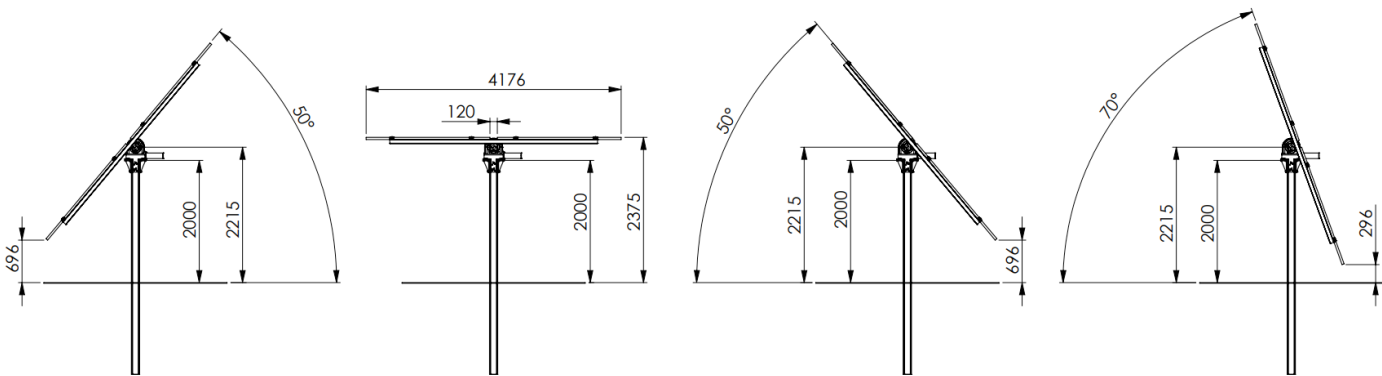
DEGER S100-PF-DR With Driven Pile Foundation (1)
