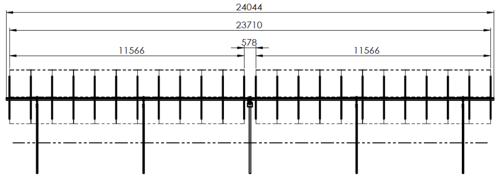
DEGER S100-DR with driven pile foundation (1)
