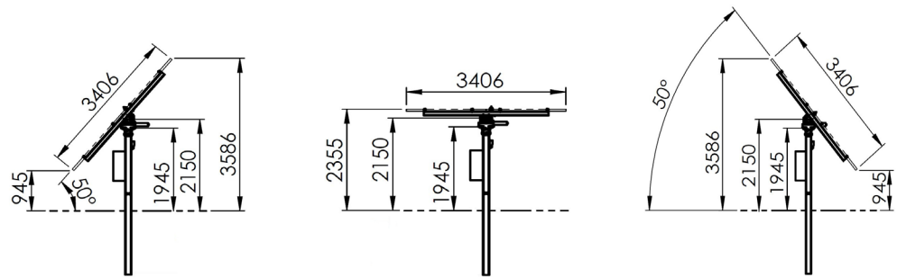
DEGER S100-DR with driven pile foundation (1)
